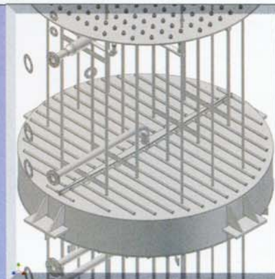
3-D SMB CAD Drawing
